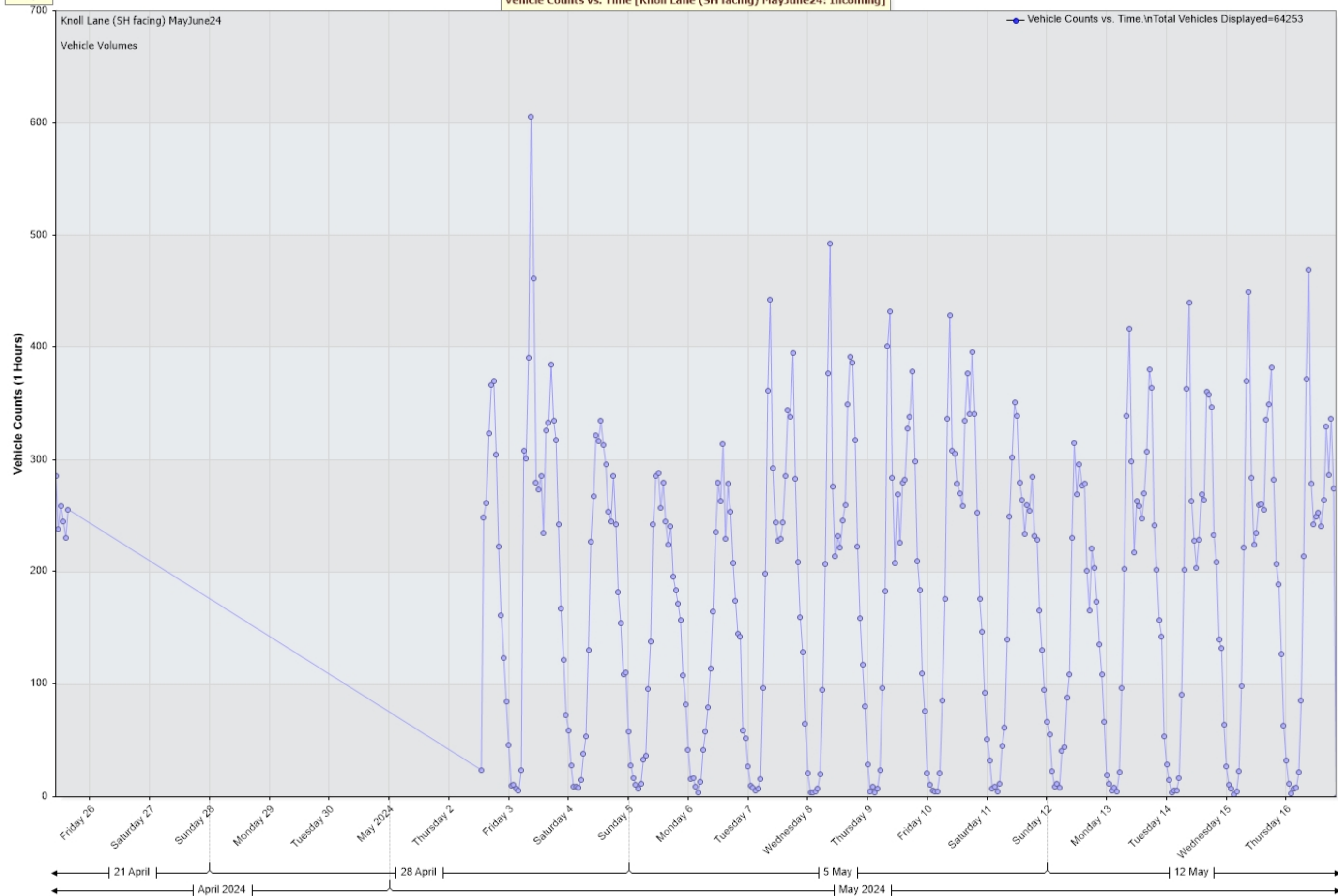
Vehicle Counts vs. Time [Knoll Lane (SH facing) MayJune24: Incoming]
