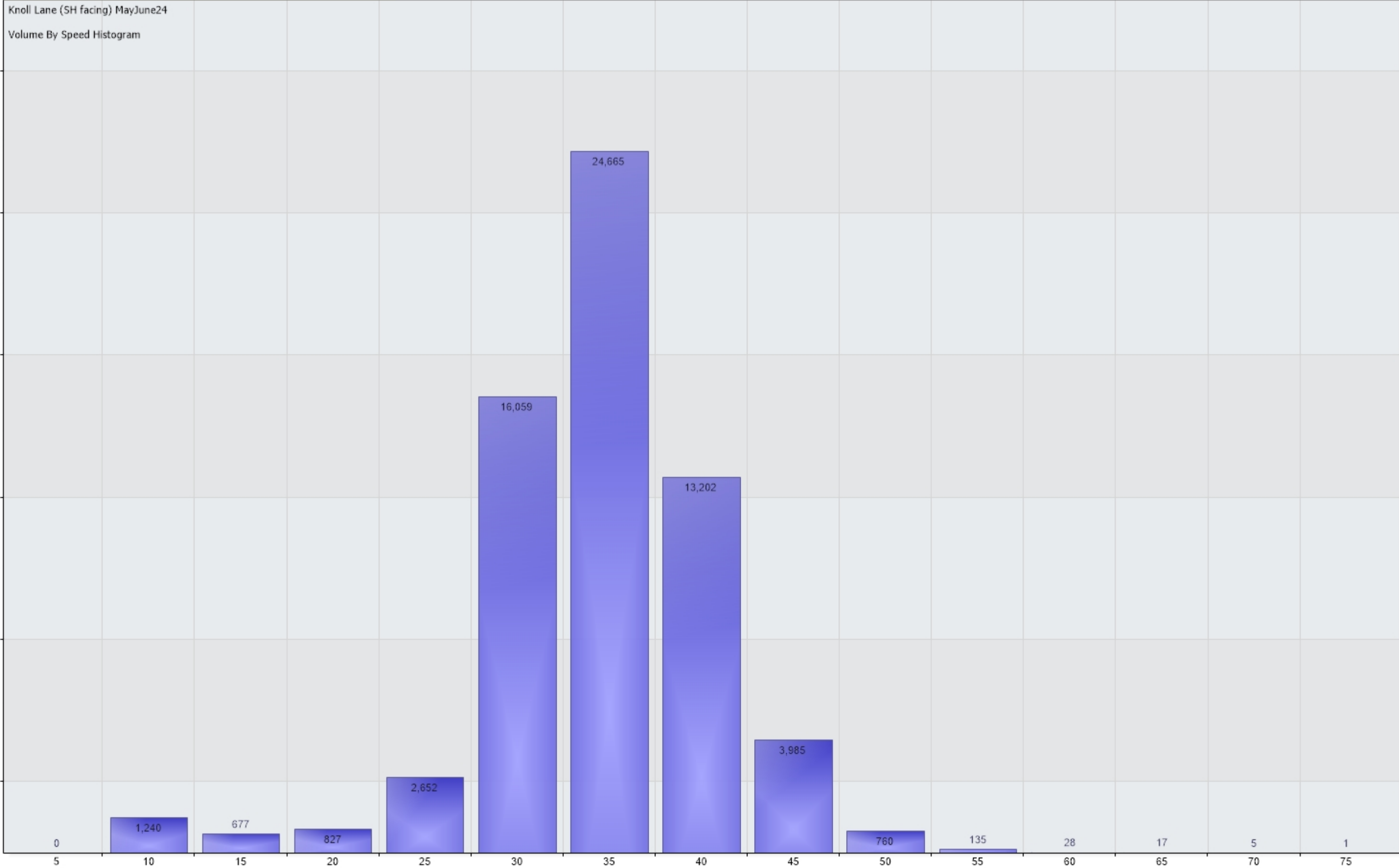
Vehicle Counts Vs. Speed [Knoll Lane (SH facing) MayJune24: Incoming]
