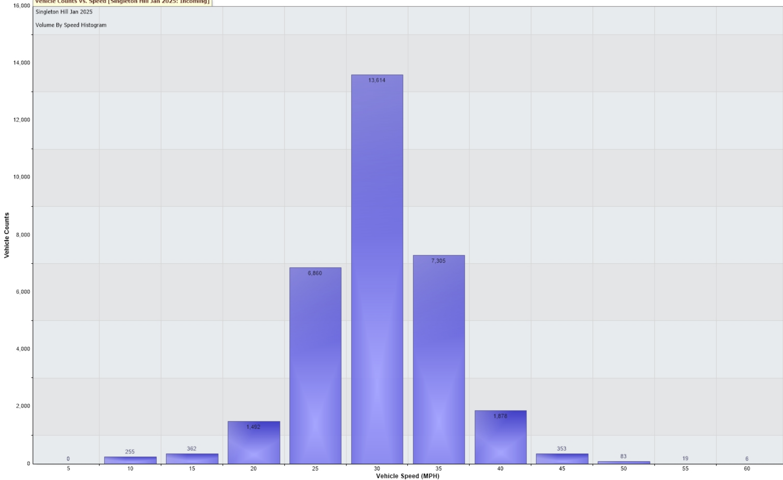
Vehicle Counts Vs. Speed [Singleton Hill Jan 2025: Incoming]
