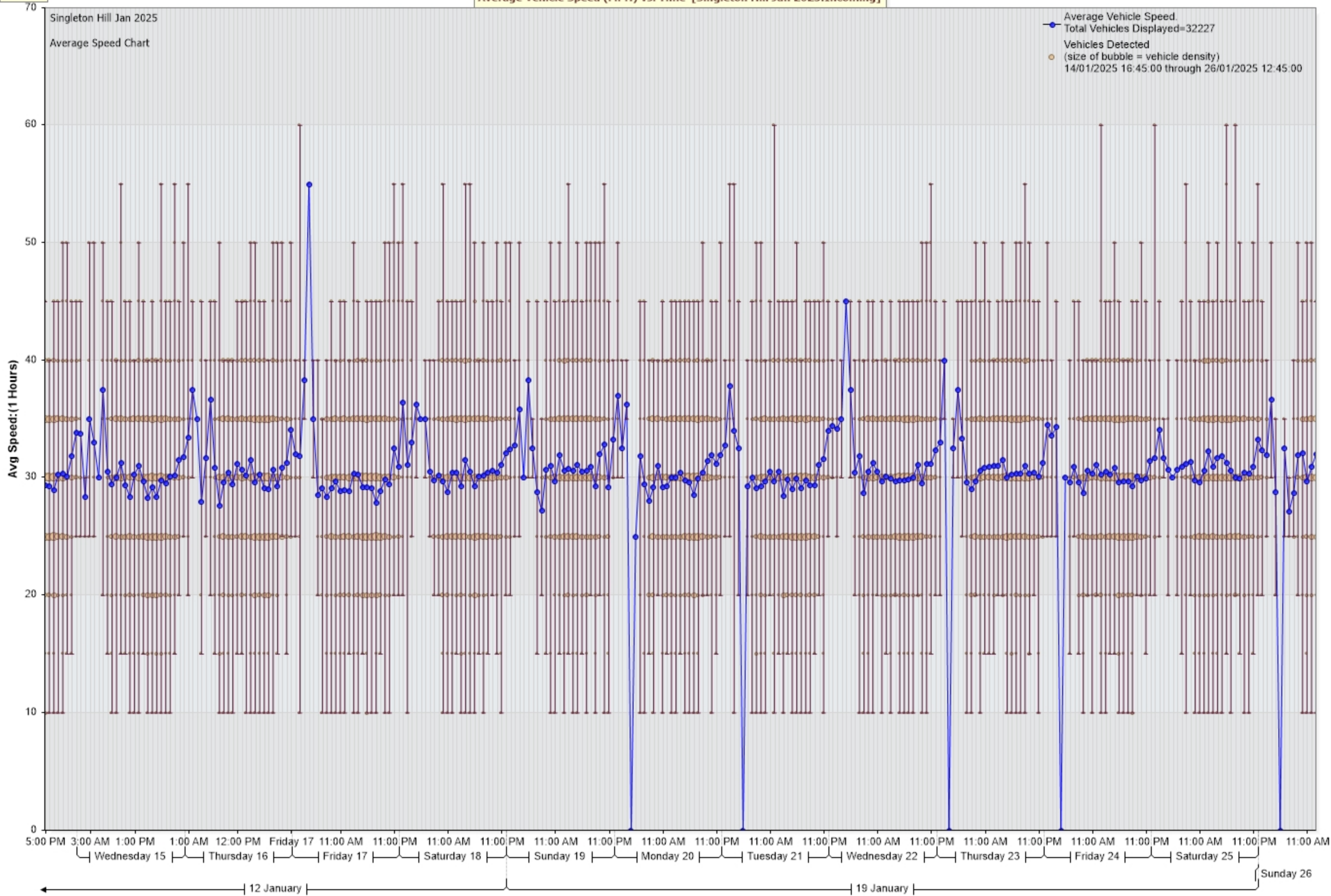
Average Vehicle Speed (MPH) vs. Time [Singleton Hill Jan 2025:Incoming]
