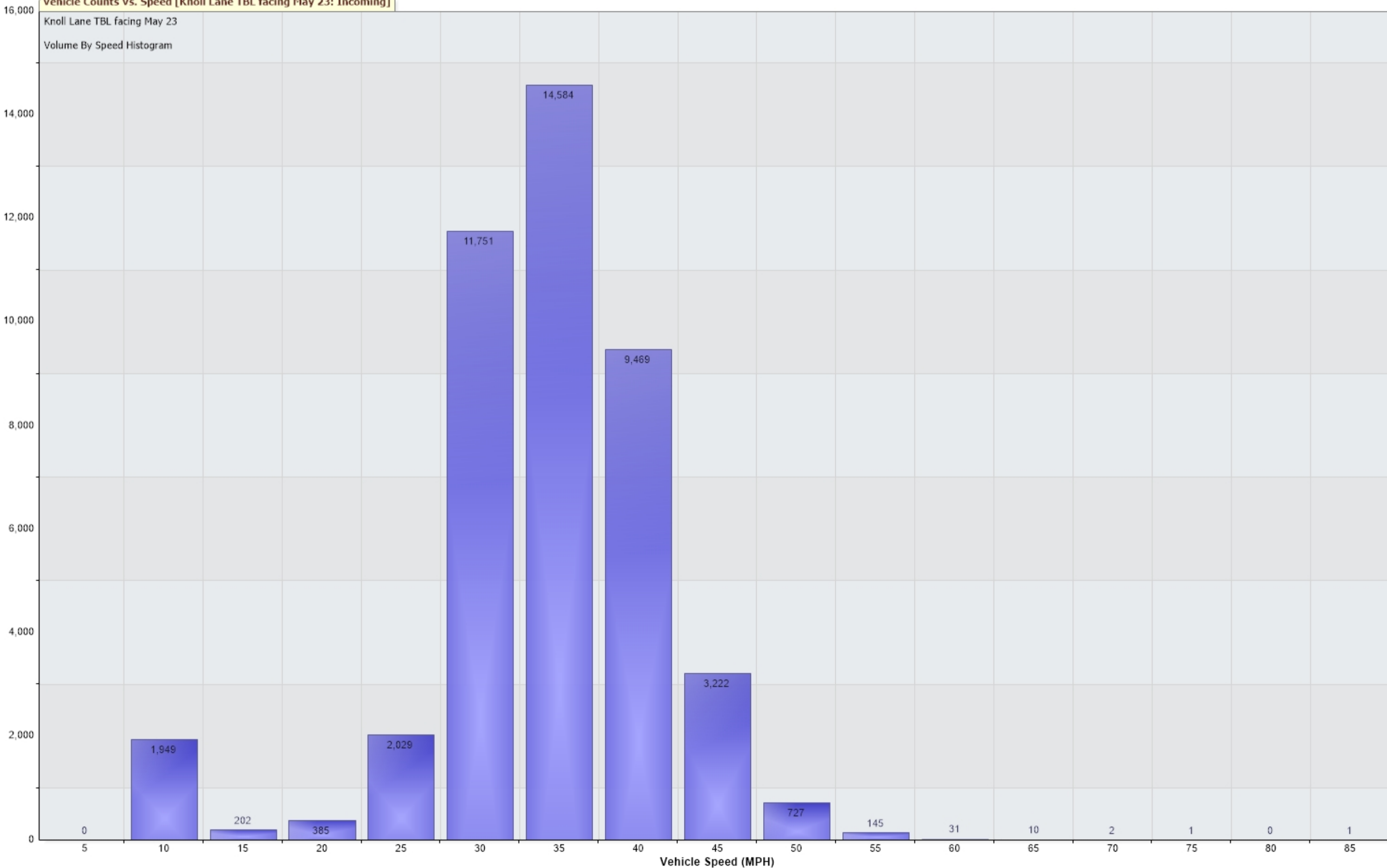
Vehicle Counts Vs. Speed [Knoll Lane TBL facing May 23: Incoming]
