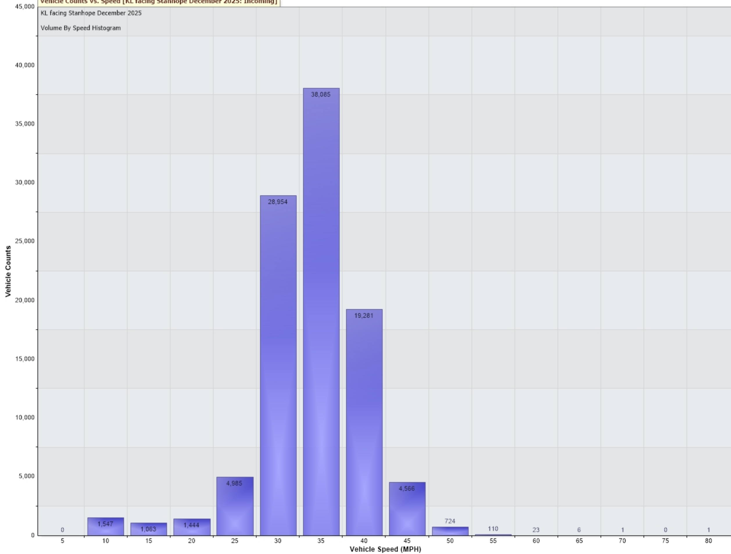
Vehicle Counts Vs. Speed [KL facing Stanhope December 2025: Incoming]
