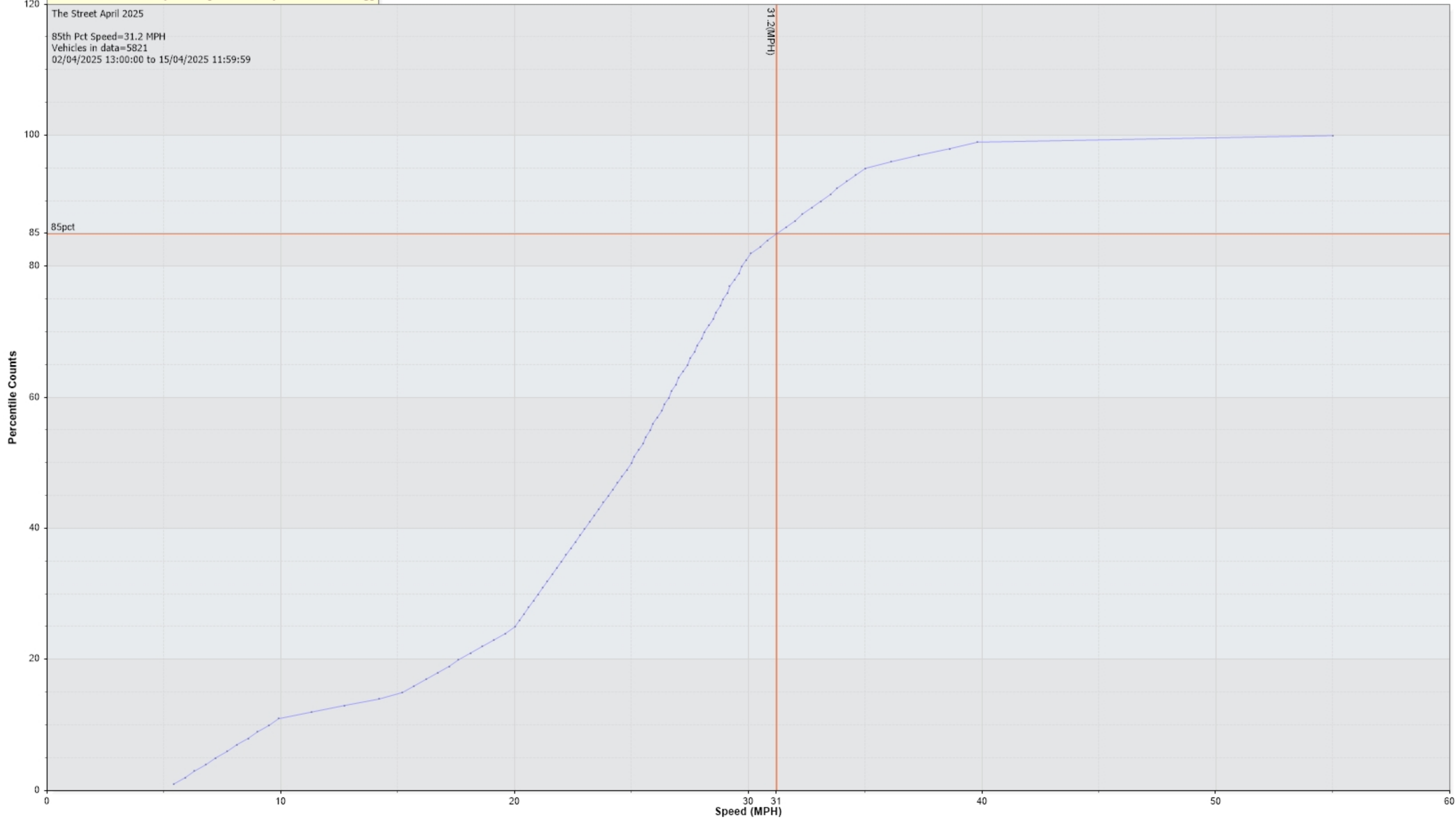
Percentile Counts Vs. Speed for [The Street April 2025: Incoming]
